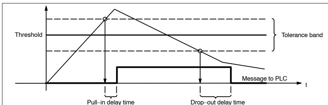
Fig. 2-6 Variable signaling function
